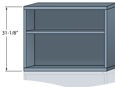
Base shelf and adjustable shelf without base channels ■ ■ N35453010500
