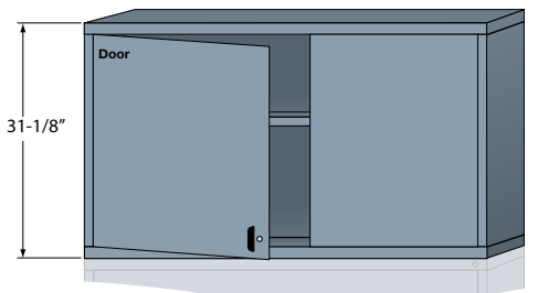
Base shelf and adjustable shelf behind lockable swing doors without base channels ■ ■ N35603010550
