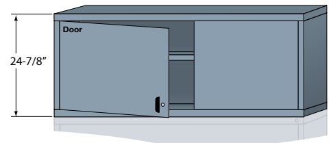
Base shelf and adjustable shelf behind lockable swing doors without base channels ■ ■ N27603010550
