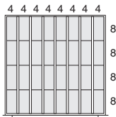
32 compartments NFOJ ___ 3030
