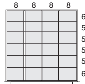
24 compartments NFOE ___ 3030
