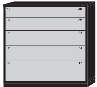
5 drawers with 86 compartments ■ ■ ■ 6860301017 ■ ■ ■
